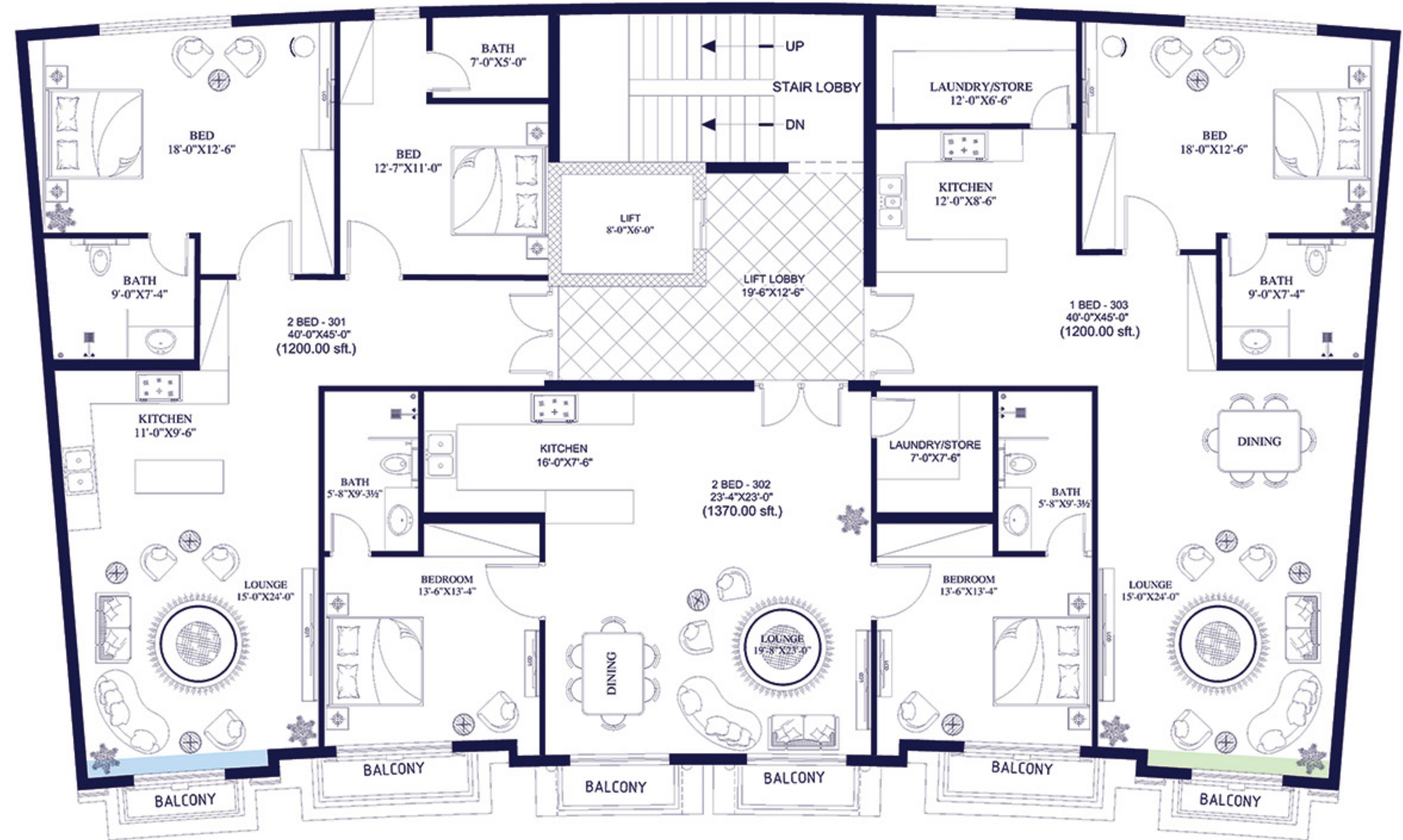
3RD FLOOR PLAN
