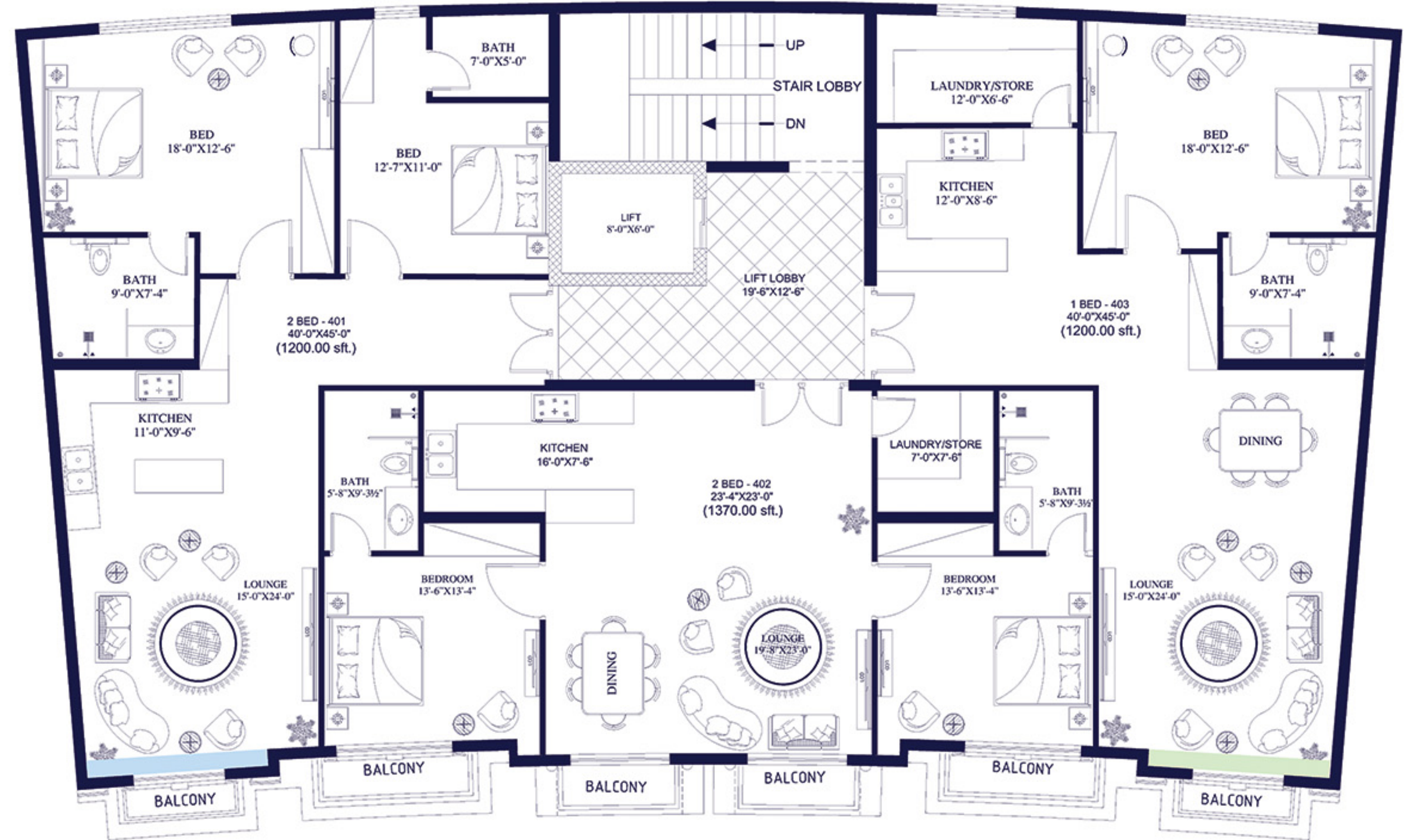
5TH FLOOR PLAN
