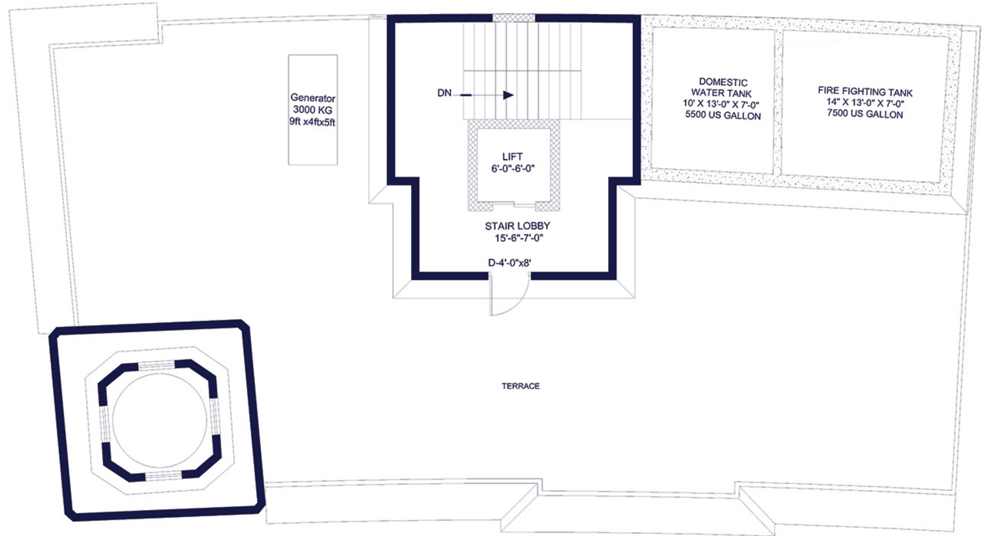
MUMTY FLOOR PLAN
