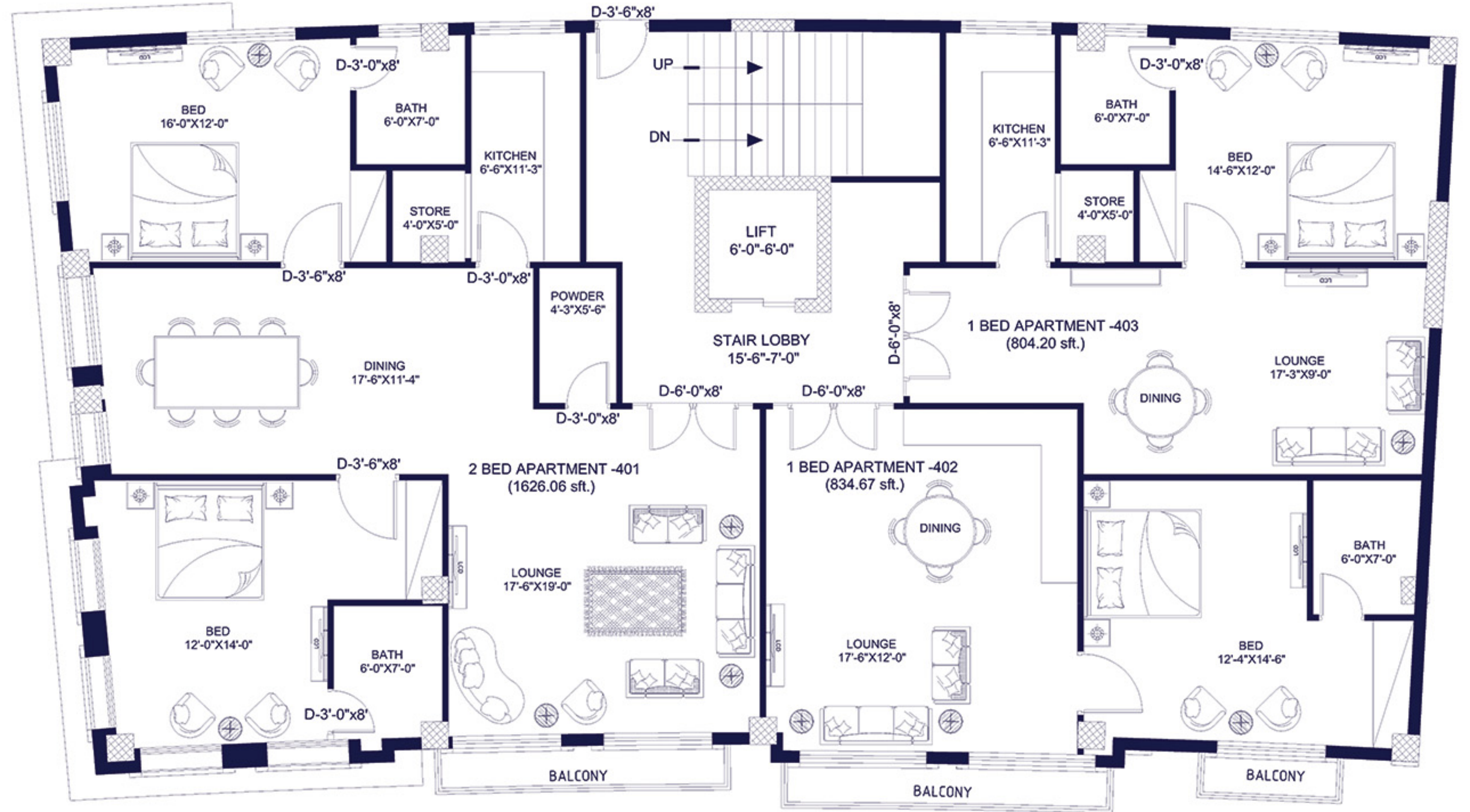
5th FLOOR PLAN
