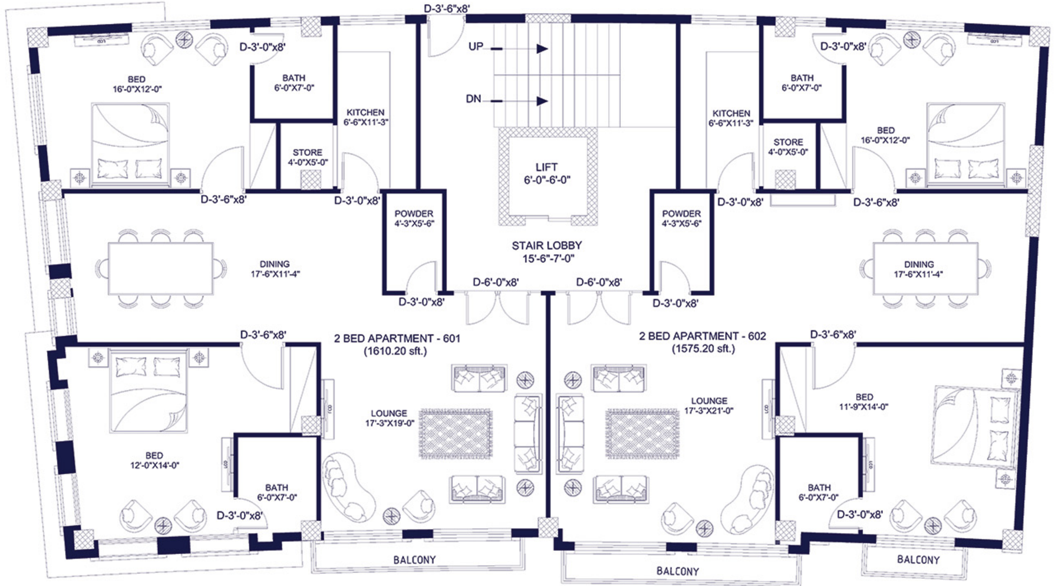
6th FLOOR PLAN
