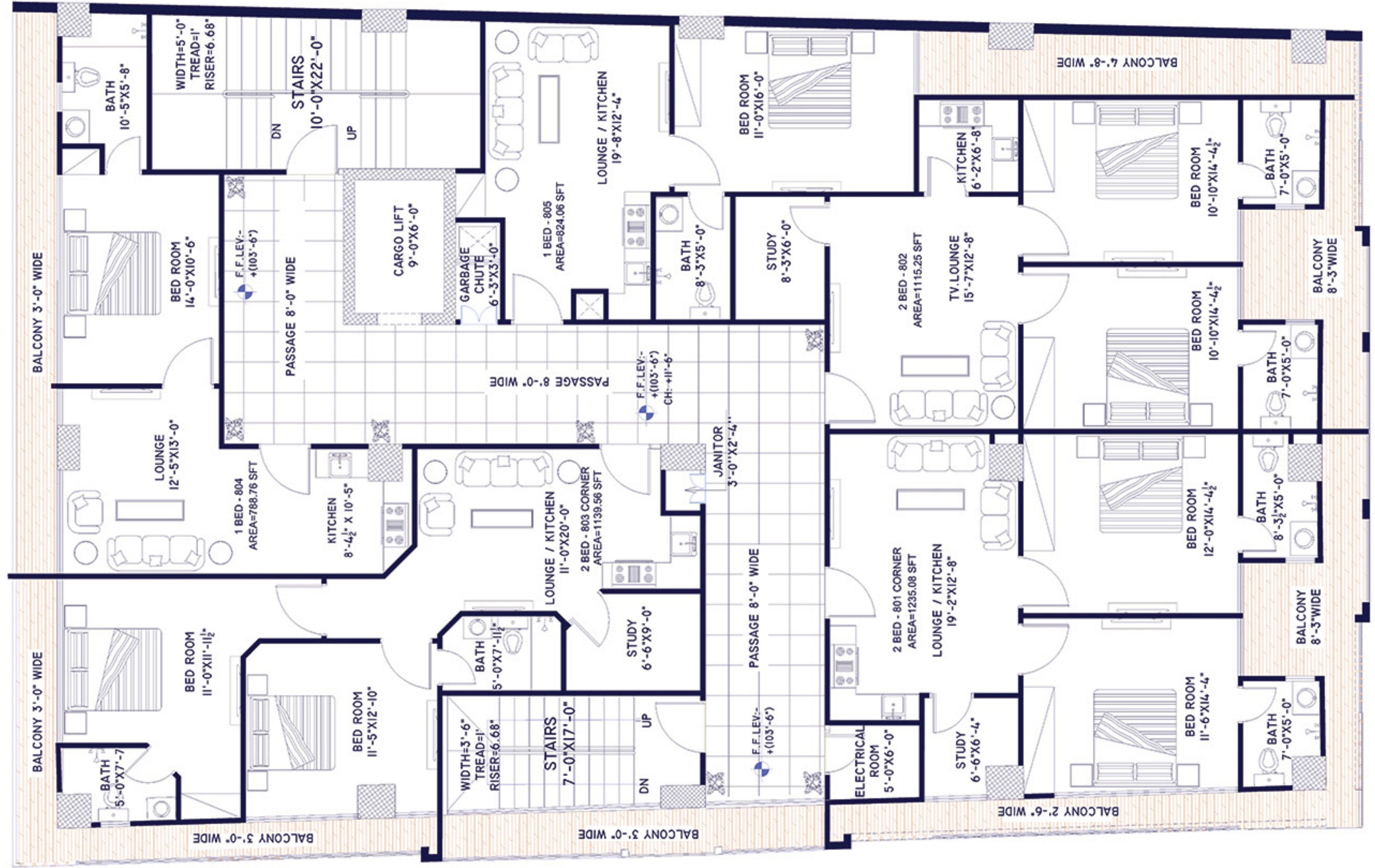
8TH FLOOR PLAN
