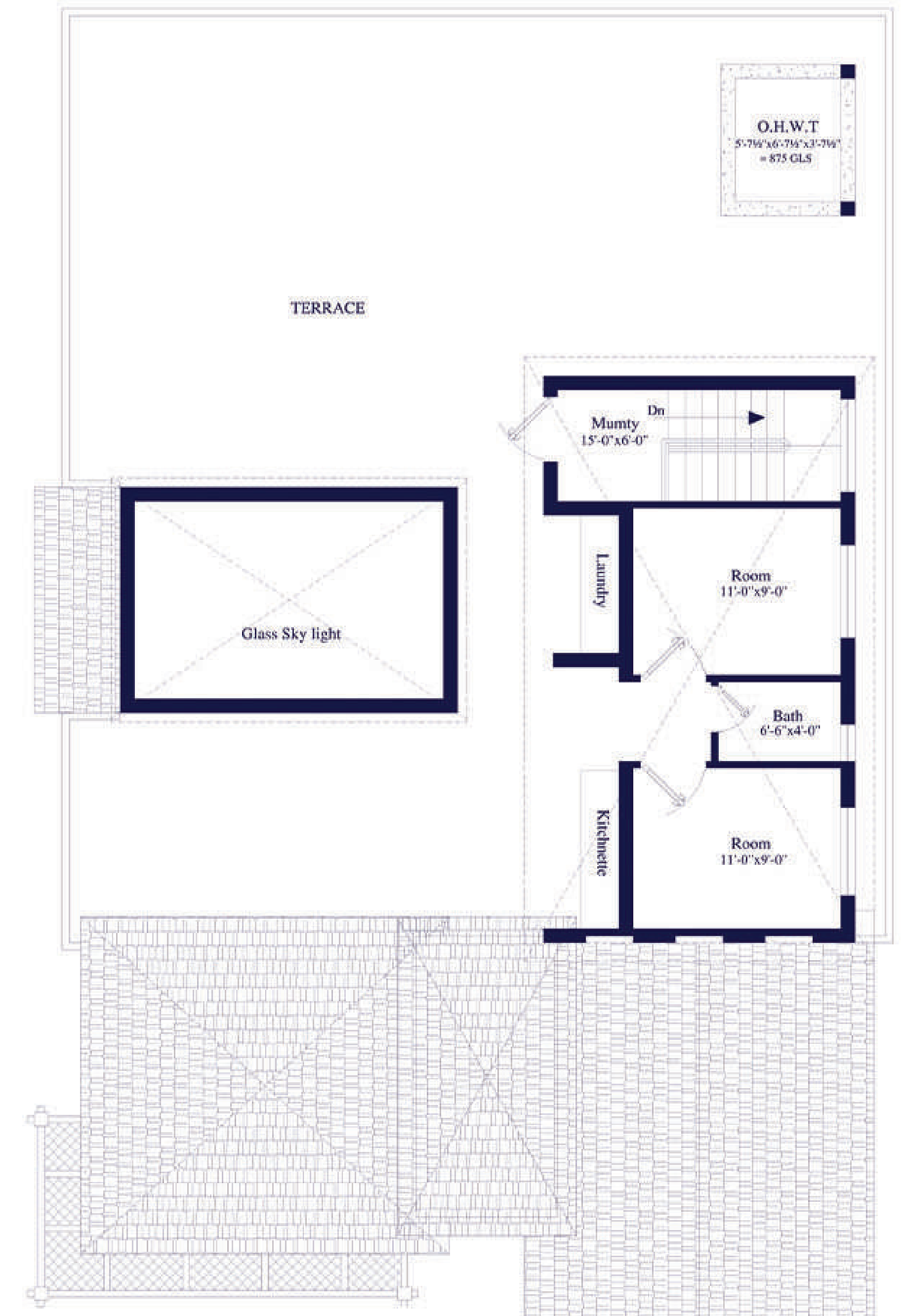
ROOF PLAN
